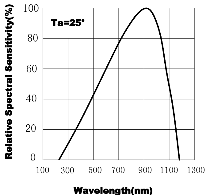
Fig.2 Spectral Sensitivity
