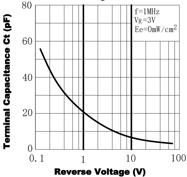
Fig.5 Terminal Capacitance vs.
