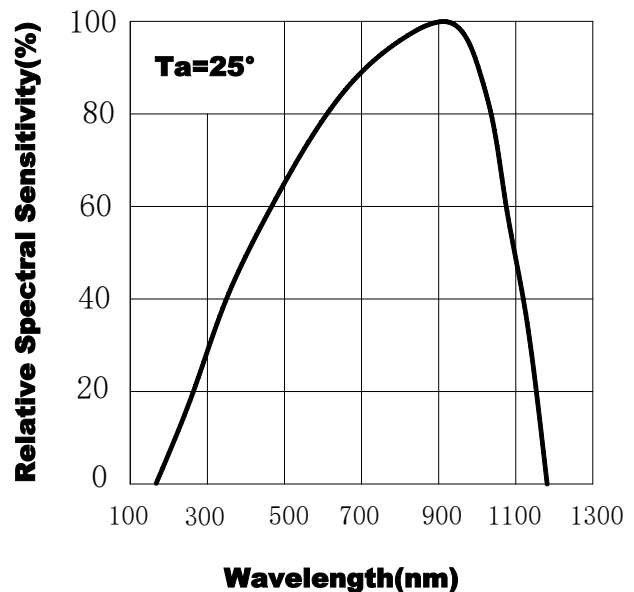
Fig.2 Spectral Sensitivity
