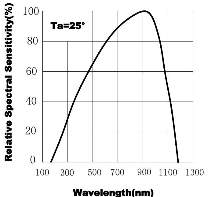
Fig.2 Spectral Sensitivity
