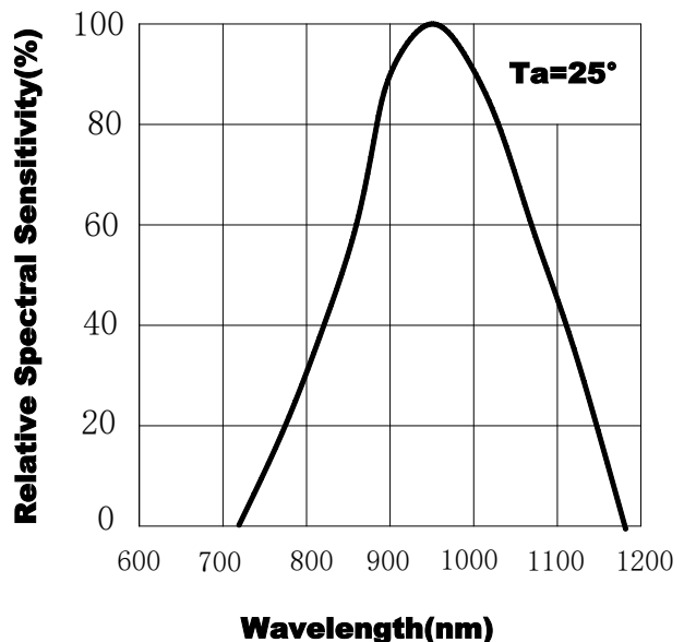
Fig.2 Spectral Sensitivity
