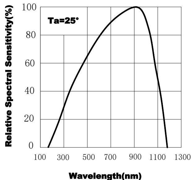
Fig.2 Spectral Sensitivity
