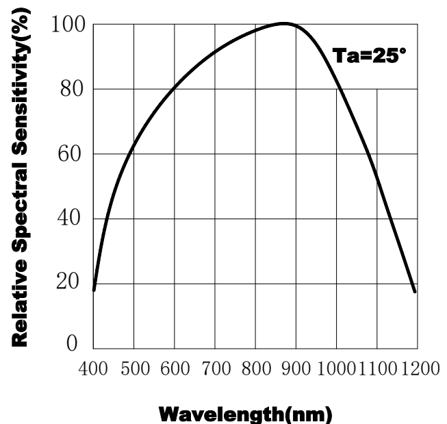
Fig.2 Spectral Sensitivity
