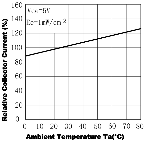
Fig.3 Relativ Collector Current vs. Ambient Temperature
