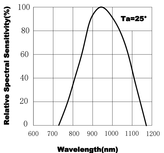
Fig.2 Spectral Sensitivity
