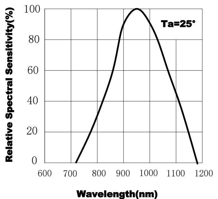
Fig.2 Spectral Sensitivity
