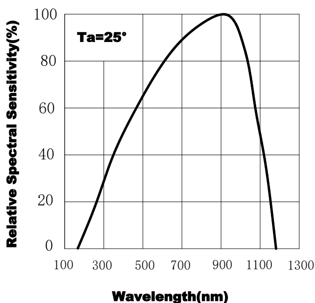
Fig.2 Spectral Sensitivity
