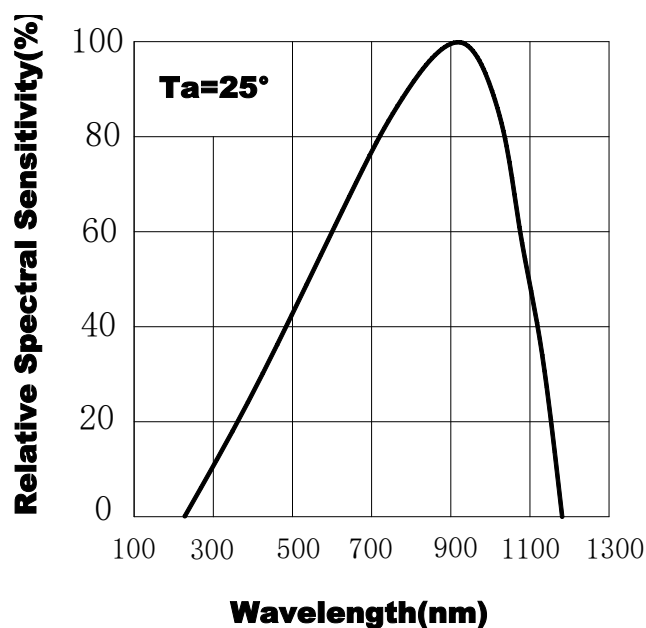
Fig.2 Spectral Sensitivity
