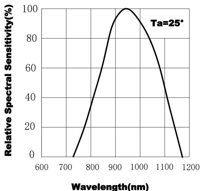
Fig.2 Spectral Sensitivity
