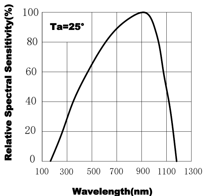
Fig.2 Spectral Sensitivity
