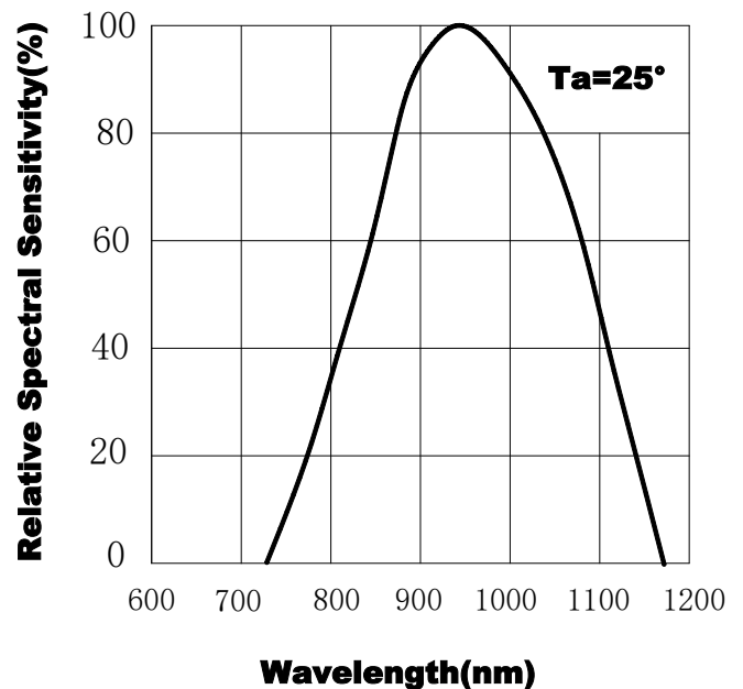
Fig.2 Spectral Sensitivity
