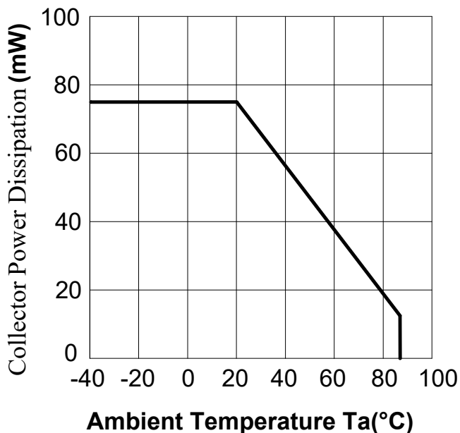
Fig.1 Collector Power Dissipation vs. Ambient Temperature
