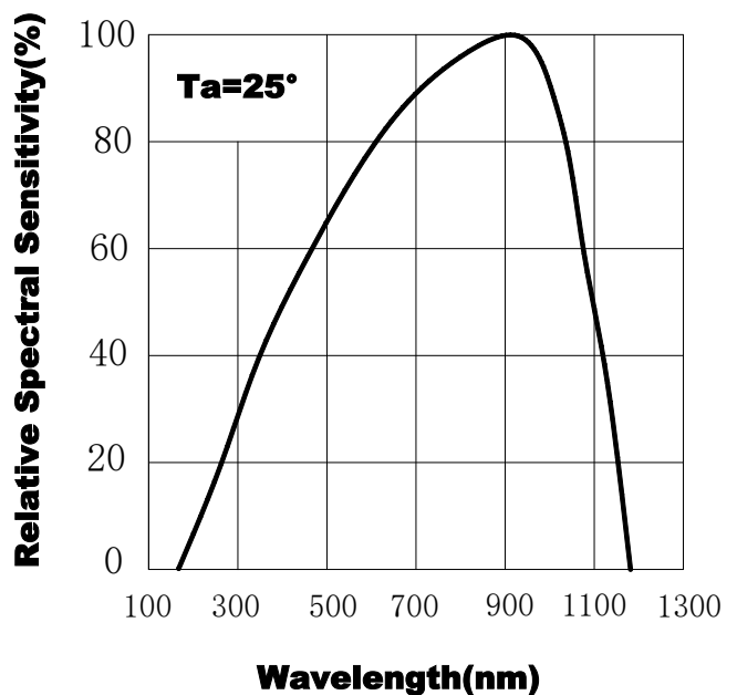
Fig.2 Spectral Sensitivity
