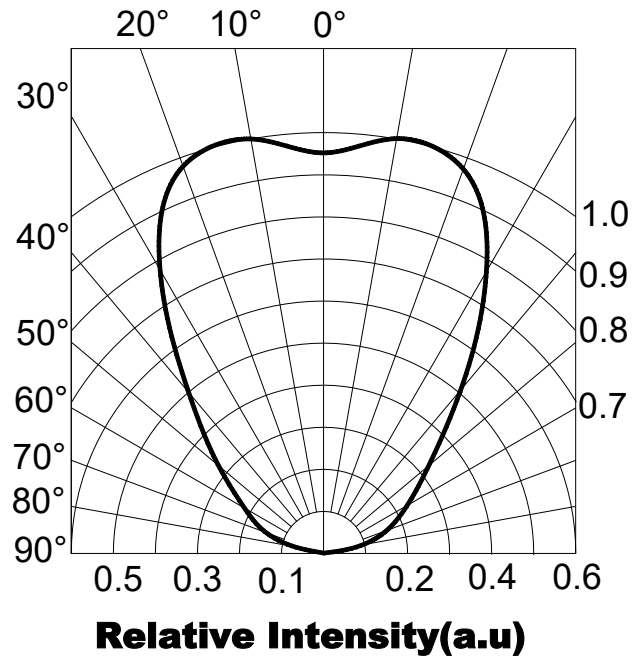
Fig.6 Relative Radiant Intensity vs. Angular Displacement
