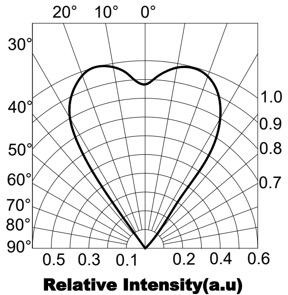
Fig.6 Relative Radiant Intensity vs. Angular Displacement
