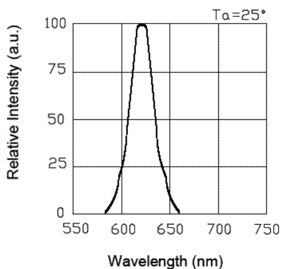
Relative Intensity vs. Wavelength (Ta=25℃)
