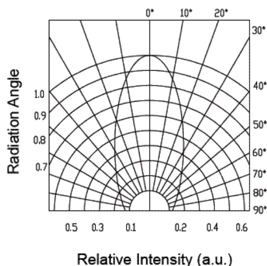
Directivity (Ta=25℃)
